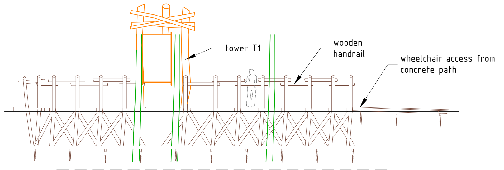
Front view
