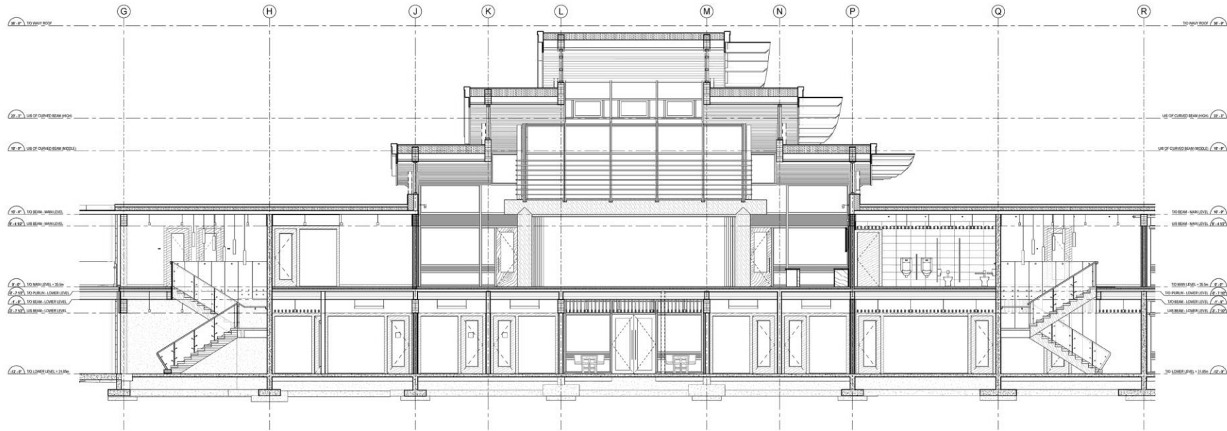
LONGITUDINAL SECTION 'L' - THROUGH MAIN WAVY ROOF 1/4" = 1'-0"
